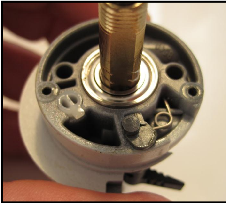
This is what the reel looks like having removed the Anti-reverse bearing
